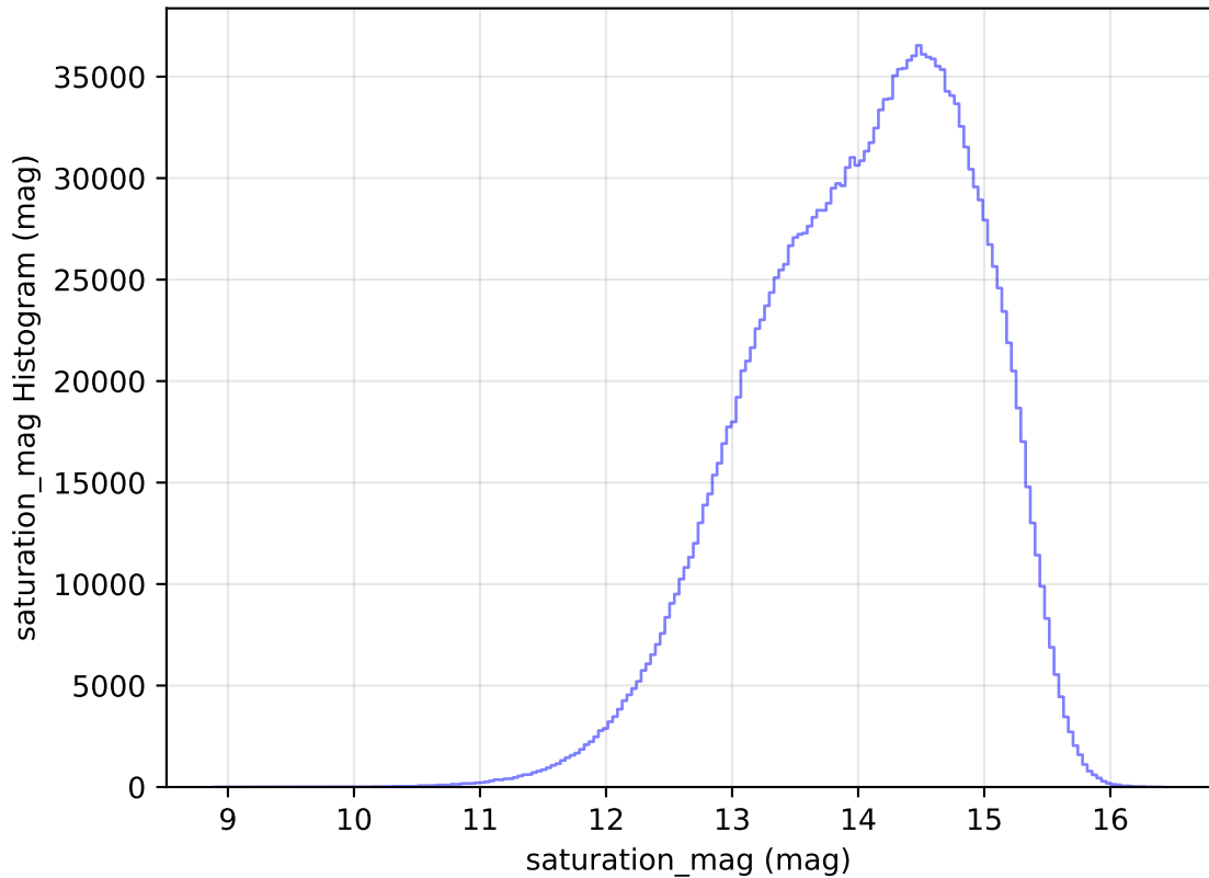
too_elab_r16_d2_griz_v3.4_10yrs WFD all bands: saturation_mag Histogram
