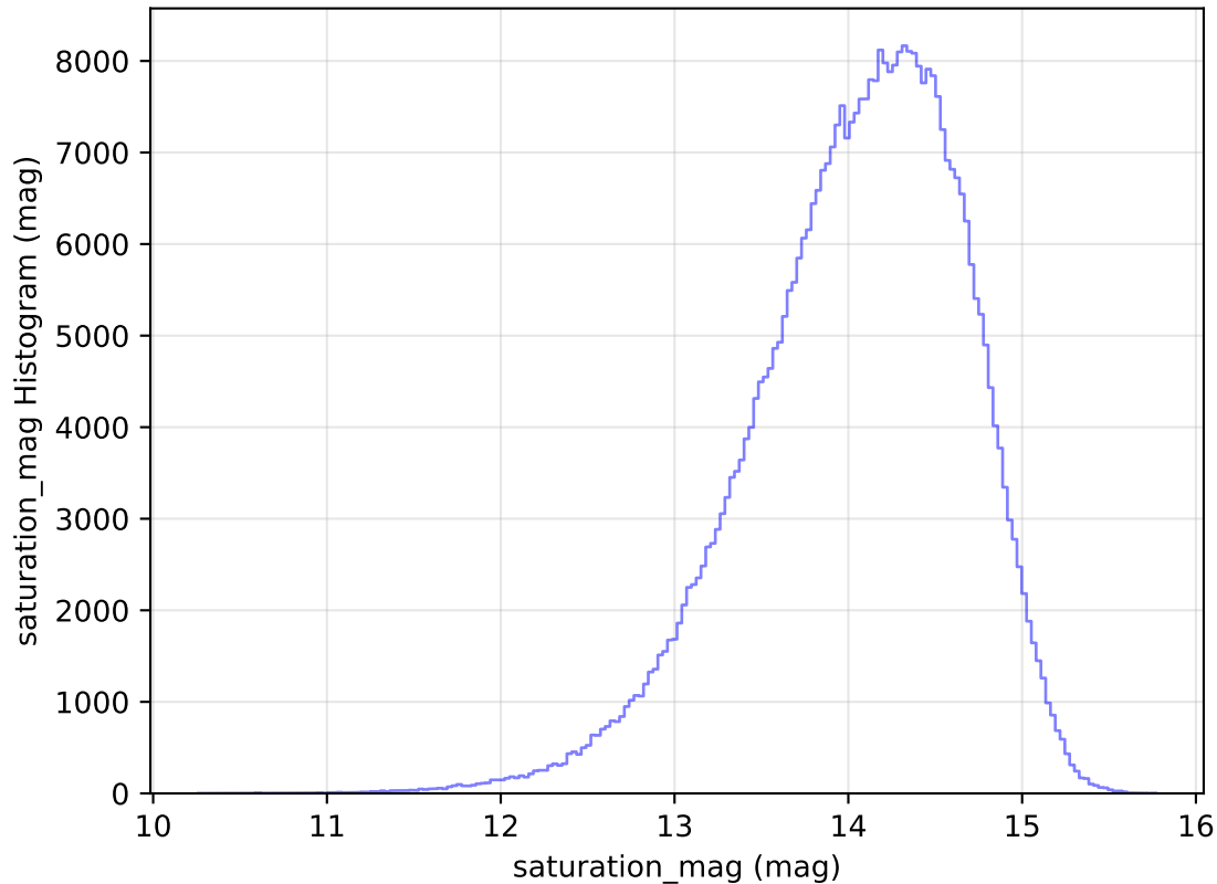
too_elab_r16_d2_griz_v3.4_10yrs All sky z band: saturation_mag Histogram
