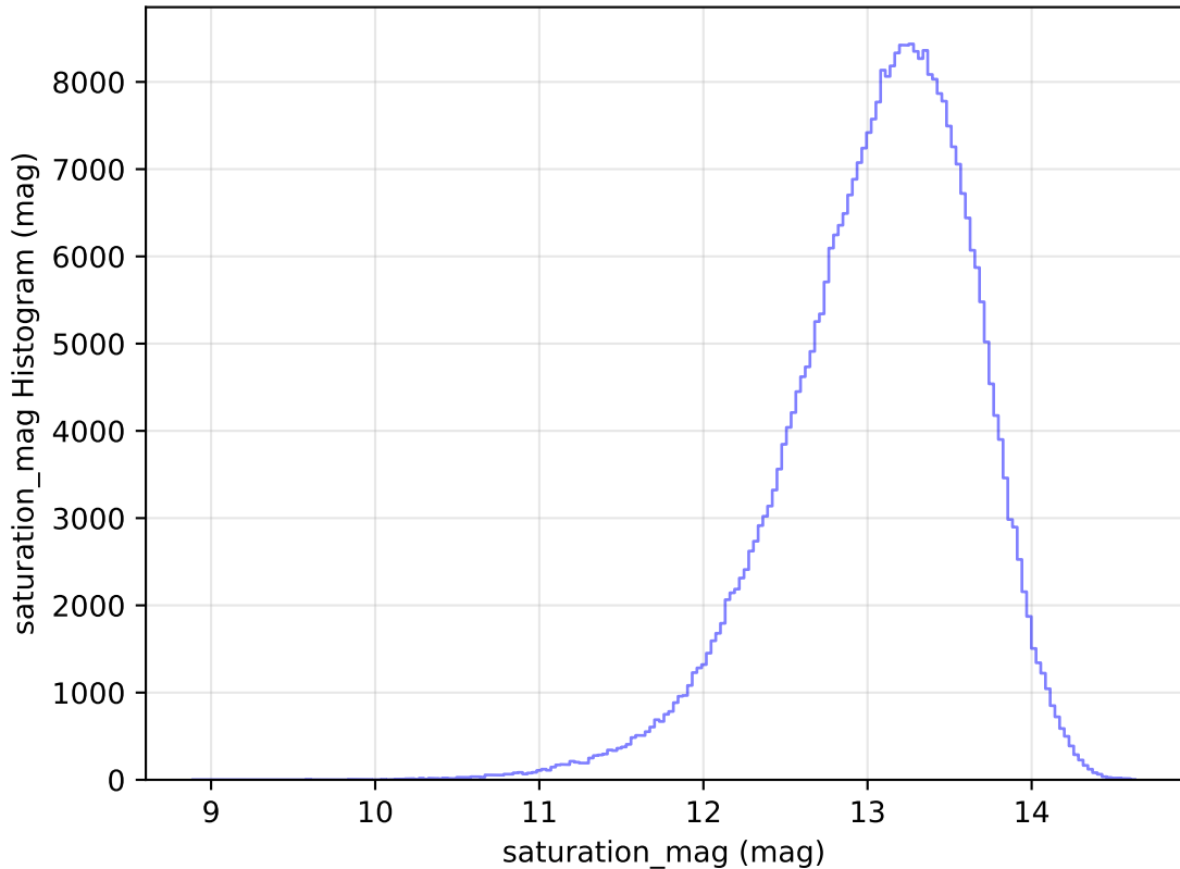
too_elab_r16_d2_griz_v3.4_10yrs All sky y band: saturation_mag Histogram
