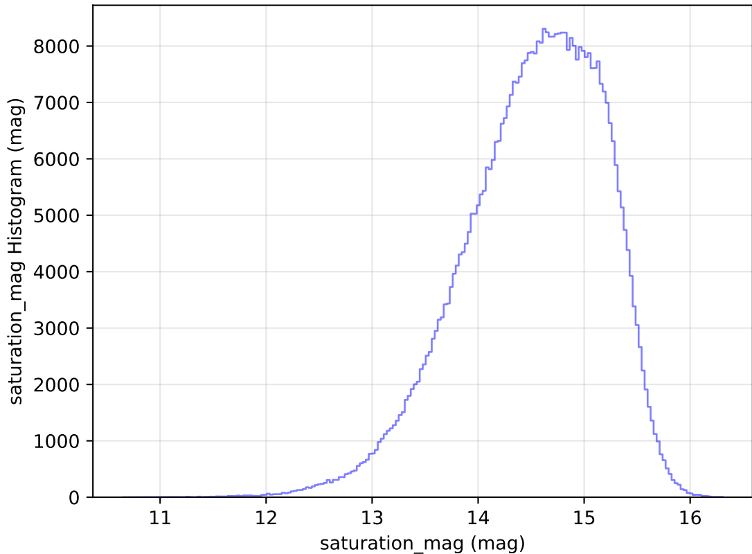
too_elab_r16_d2_griz_v3.4_10yrs All sky r band: saturation_mag Histogram
