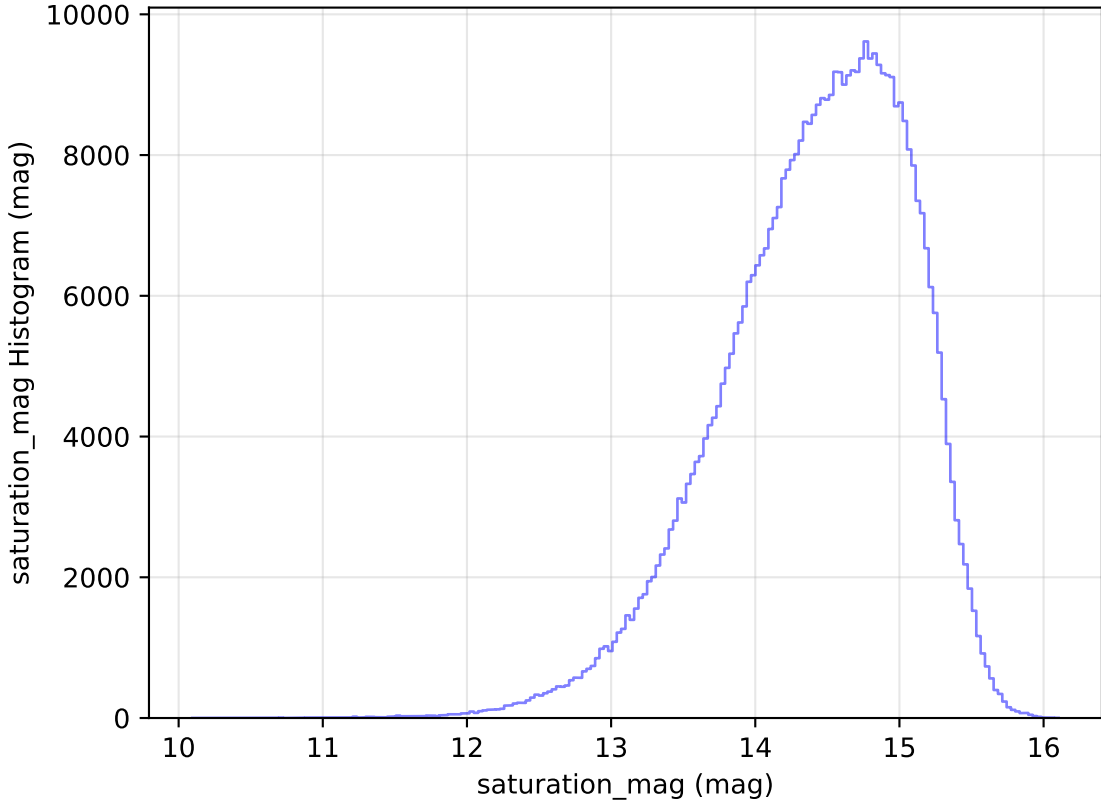
too_elab_r16_d2_griz_v3.4_10yrs All sky i band: saturation_mag Histogram
