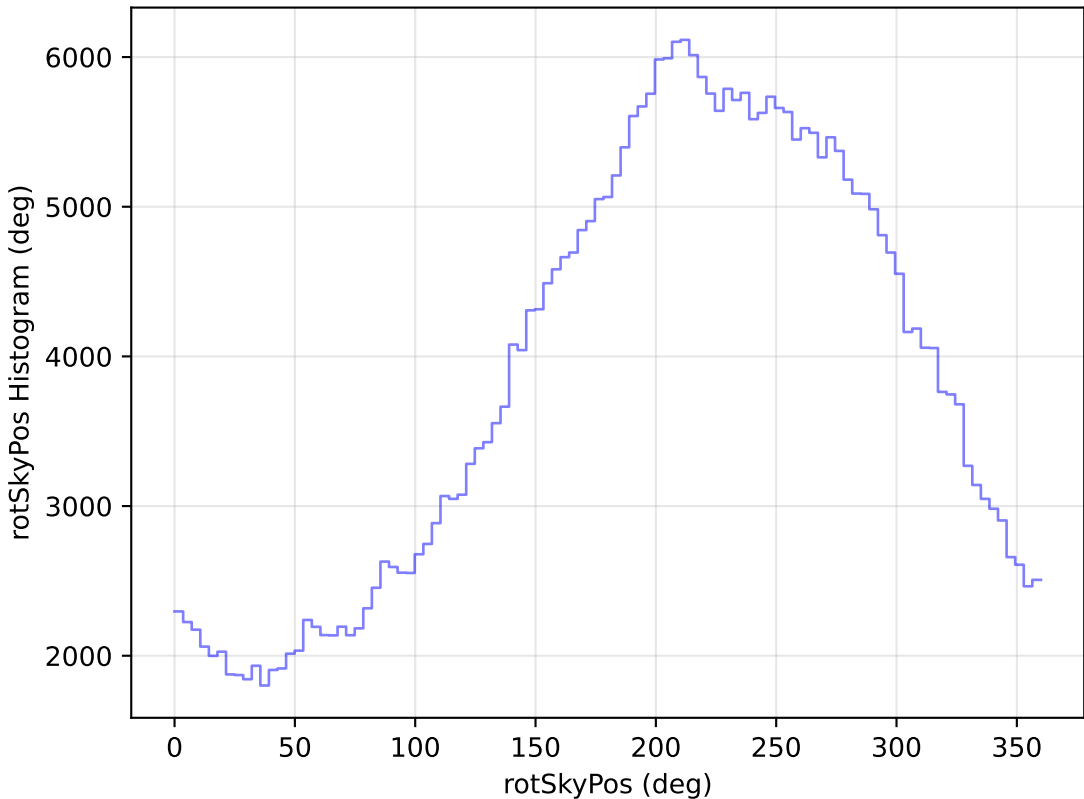
too_elab_r16_d2_griz_v3.4_10yrs WFD y band: rotSkyPos Histogram
