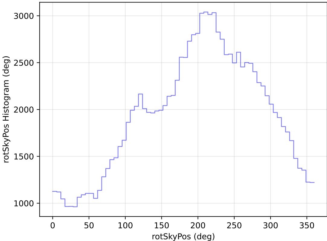
too_elab_r16_d2_griz_v3.4_10yrs WFD u band: rotSkyPos Histogram
