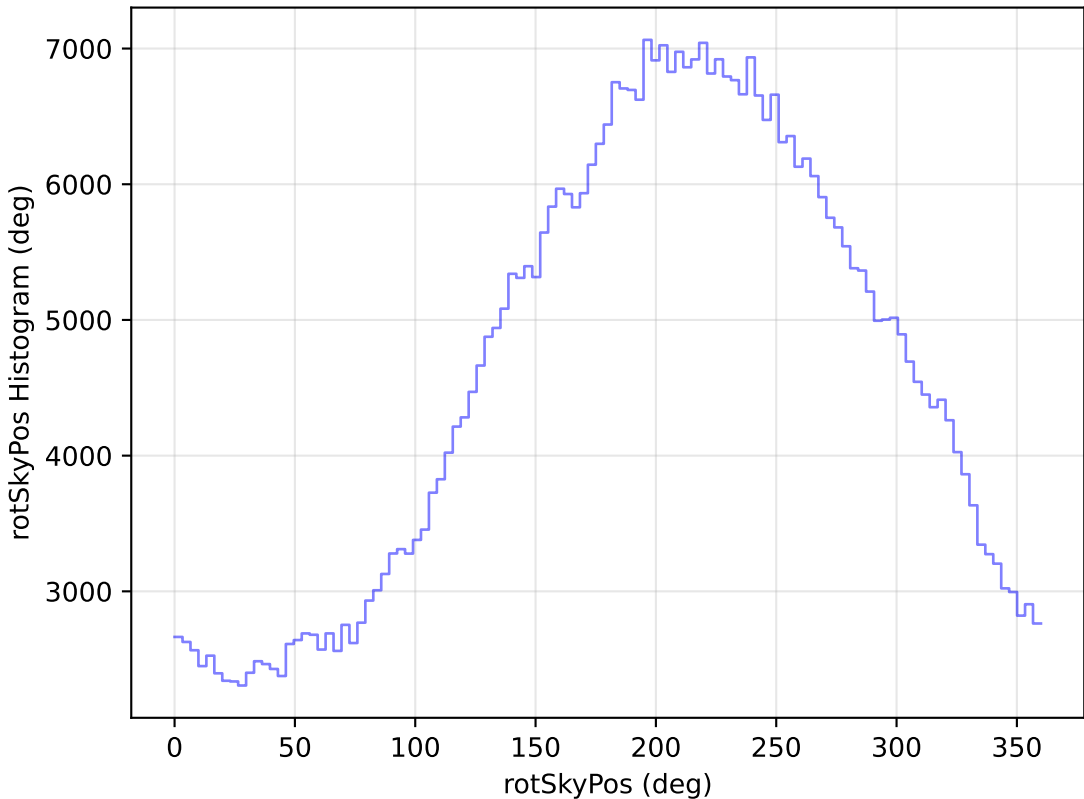
too_elab_r16_d2_griz_v3.4_10yrs WFD i band: rotSkyPos Histogram
