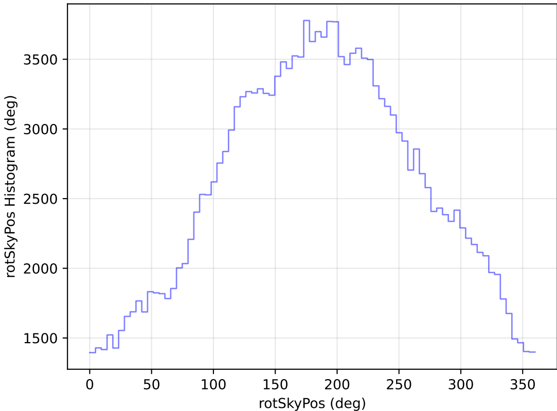
too_elab_r16_d2_griz_v3.4_10yrs WFD g band: rotSkyPos Histogram
