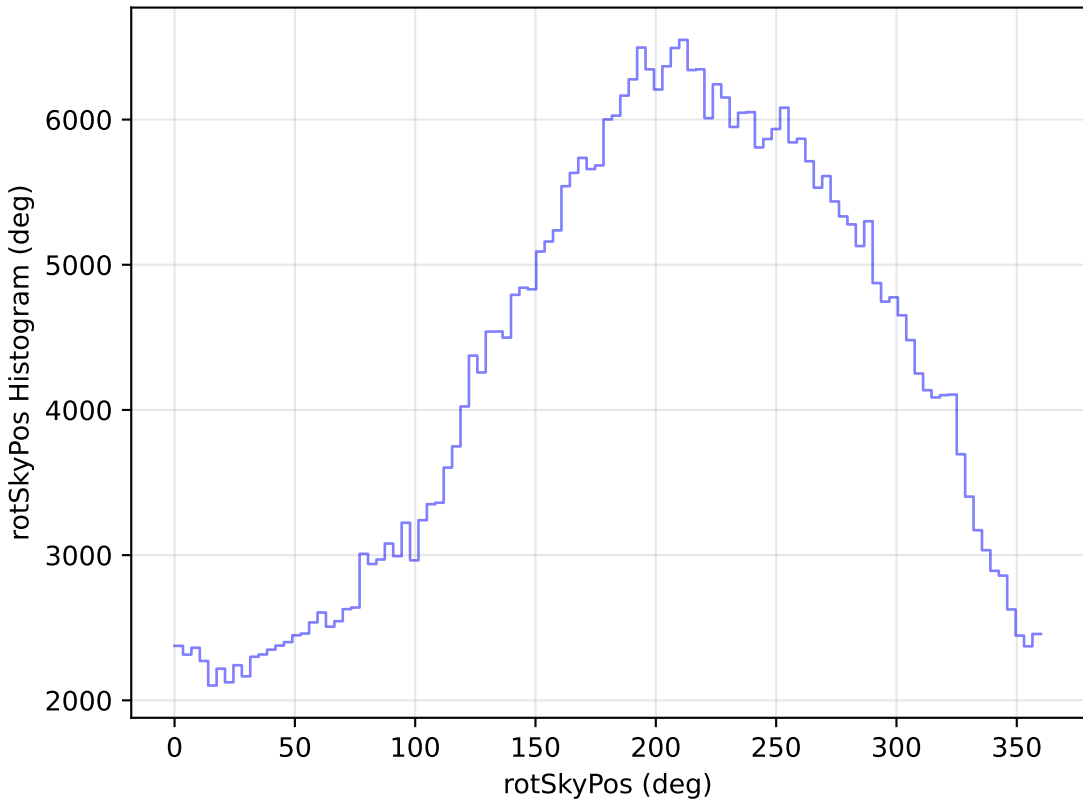
too_elab_r16_d2_griz_v3.4_10yrs All sky z band: rotSkyPos Histogram
