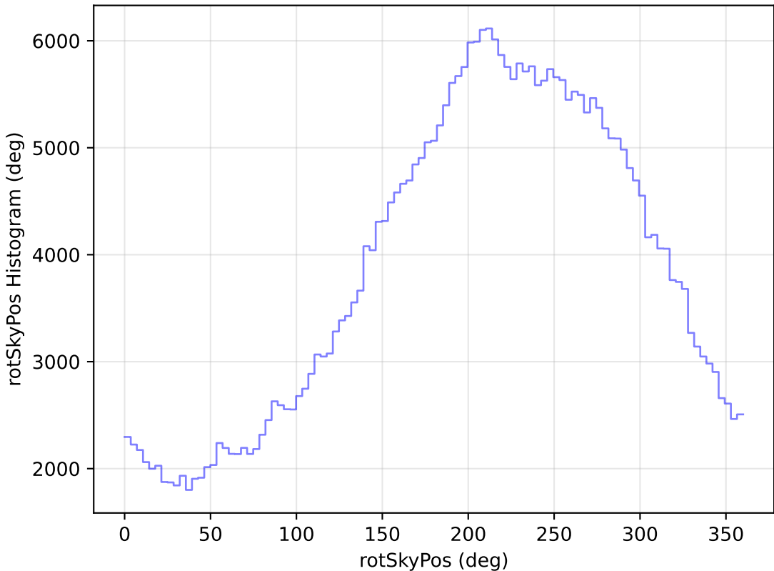
too_elab_r16_d2_griz_v3.4_10yrs All sky y band: rotSkyPos Histogram
