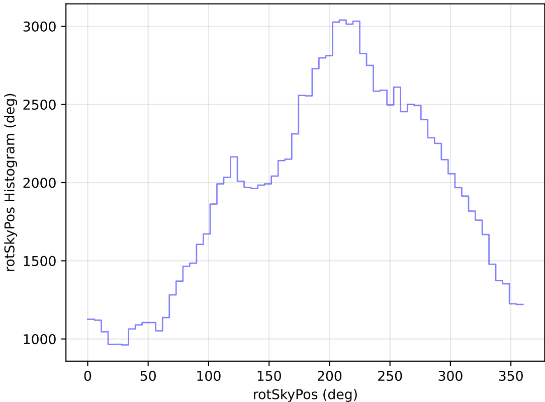
too_elab_r16_d2_griz_v3.4_10yrs All sky u band: rotSkyPos Histogram
