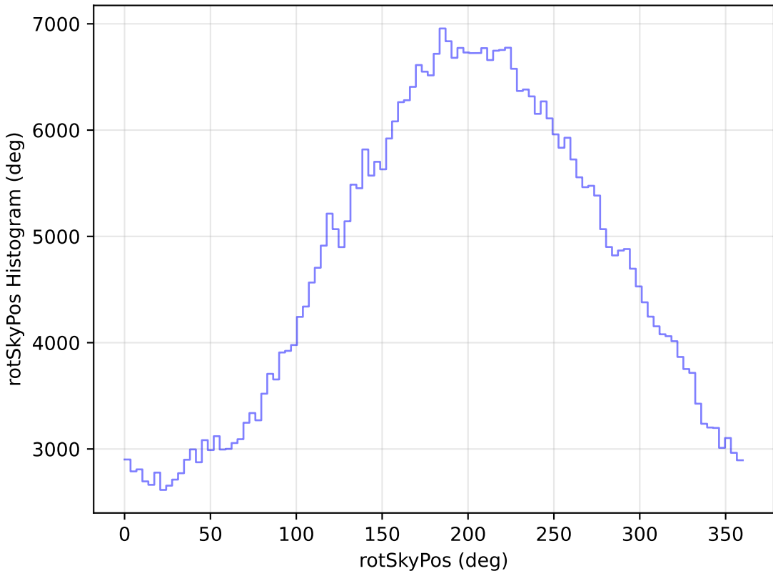
too_elab_r16_d2_griz_v3.4_10yrs All sky r band: rotSkyPos Histogram
