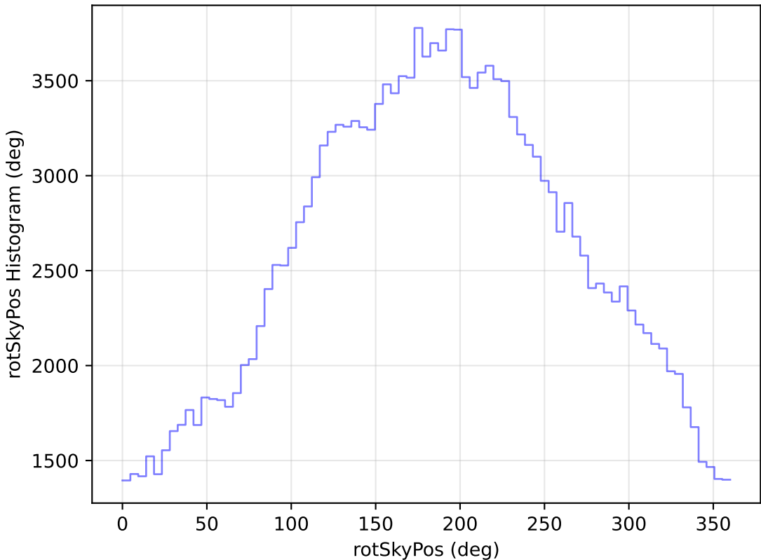
too_elab_r16_d2_griz_v3.4_10yrs All sky g band: rotSkyPos Histogram
