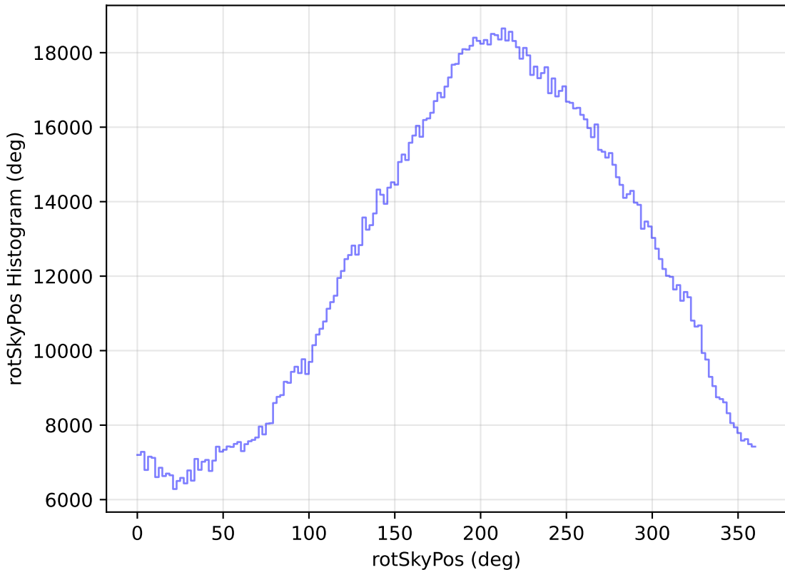
too_elab_r16_d2_griz_v3.4_10yrs All sky all bands: rotSkyPos Histogram
