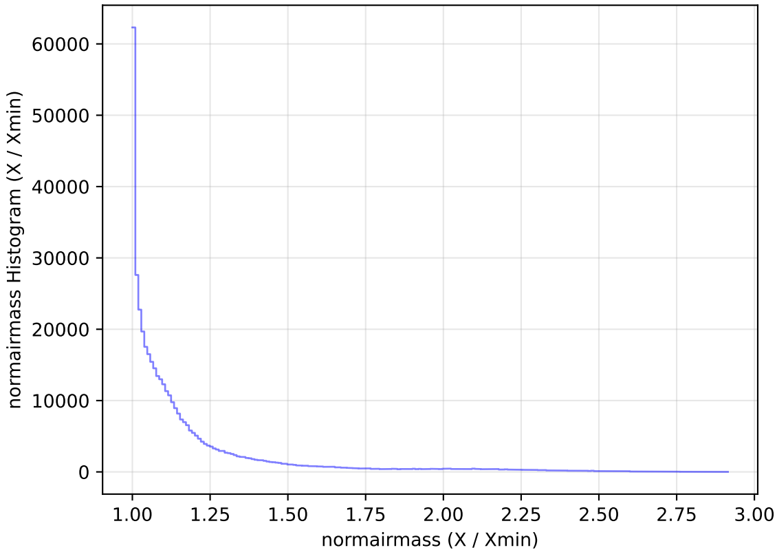
too_elab_r16_d2_griz_v3.4_10yrs WFD z band: normairmass Histogram
