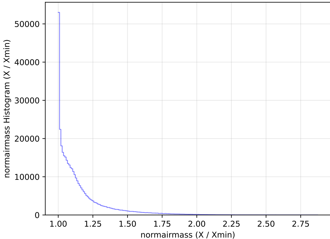
too_elab_r16_d2_griz_v3.4_10yrs WFD y band: normairmass Histogram
