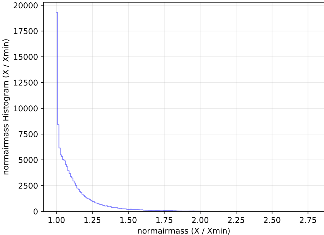
too_elab_r16_d2_griz_v3.4_10yrs WFD u band: normairmass Histogram
