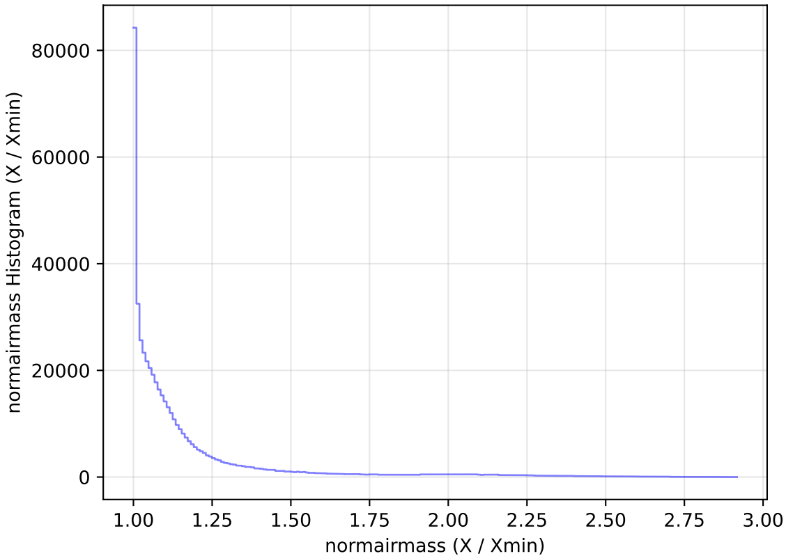
too_elab_r16_d2_griz_v3.4_10yrs WFD i band: normairmass Histogram
