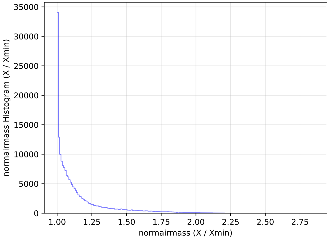
too_elab_r16_d2_griz_v3.4_10yrs WFD g band: normairmass Histogram
