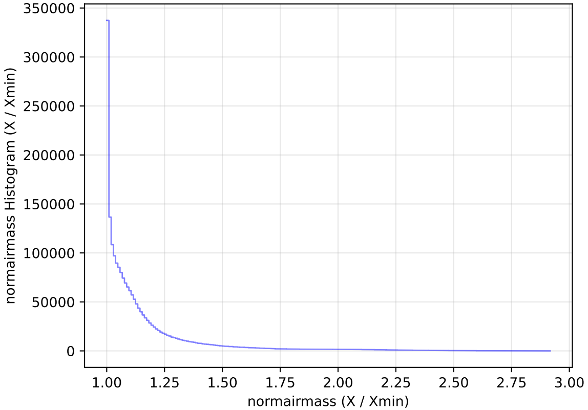
too_elab_r16_d2_griz_v3.4_10yrs WFD all bands: normairmass Histogram
