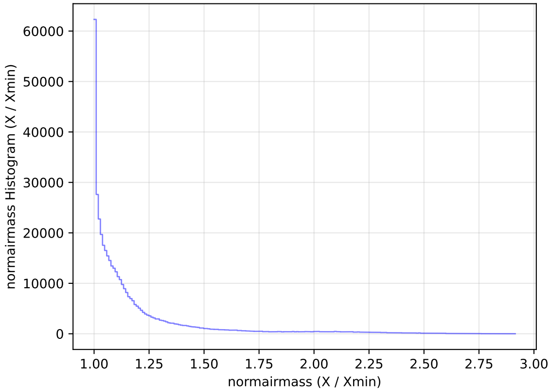
too_elab_r16_d2_griz_v3.4_10yrs All sky z band: normairmass Histogram
