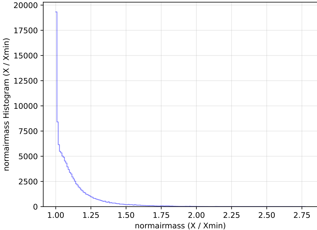
too_elab_r16_d2_griz_v3.4_10yrs All sky u band: normairmass Histogram
