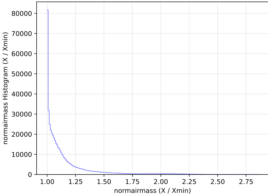
too_elab_r16_d2_griz_v3.4_10yrs All sky r band: normairmass Histogram
