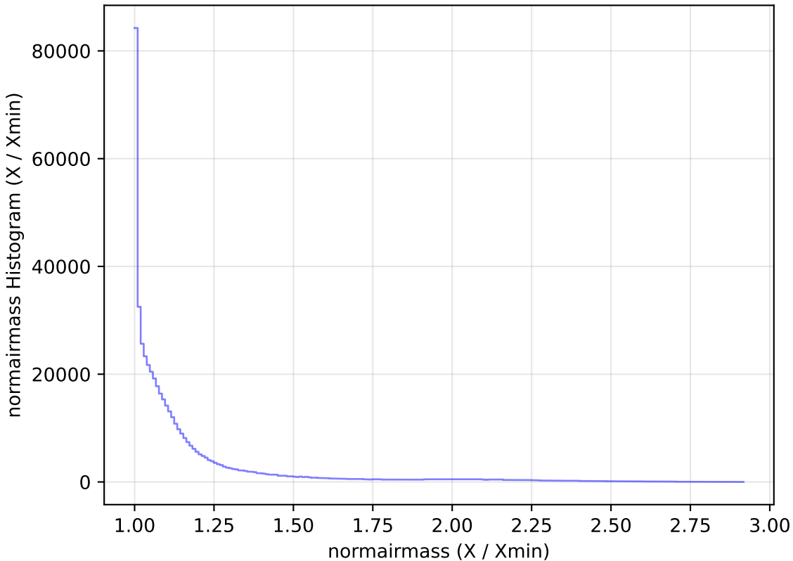
too_elab_r16_d2_griz_v3.4_10yrs All sky i band: normairmass Histogram
