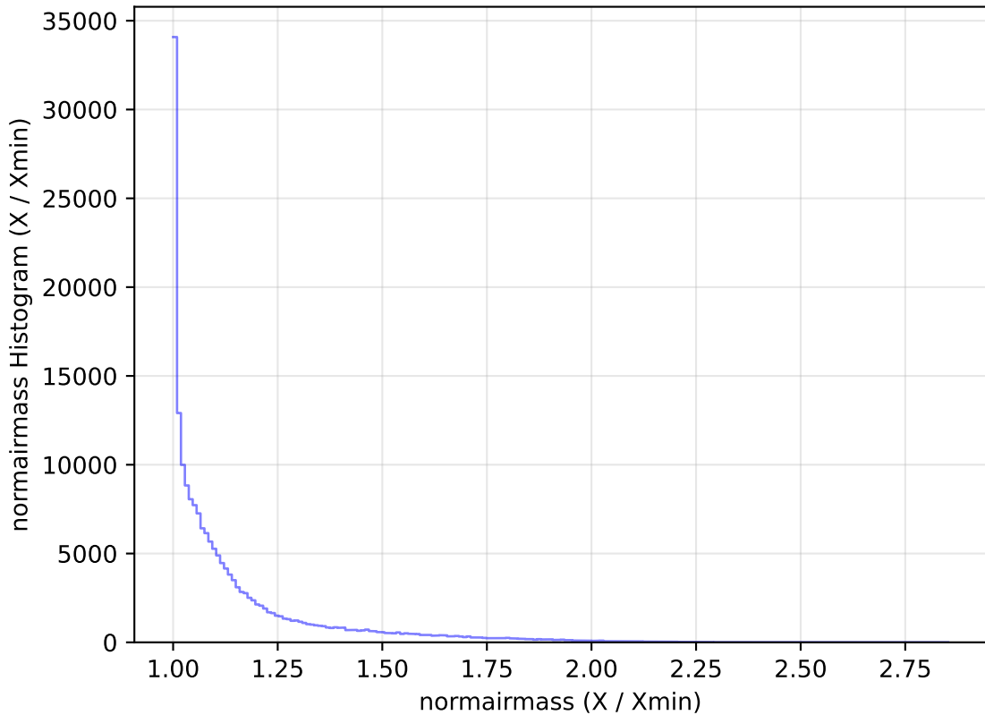
too_elab_r16_d2_griz_v3.4_10yrs All sky g band: normairmass Histogram
