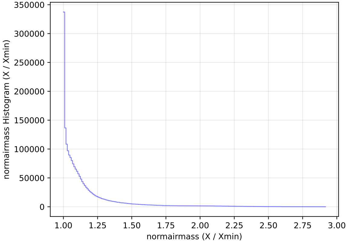
too_elab_r16_d2_griz_v3.4_10yrs All sky all bands: normairmass Histogram
