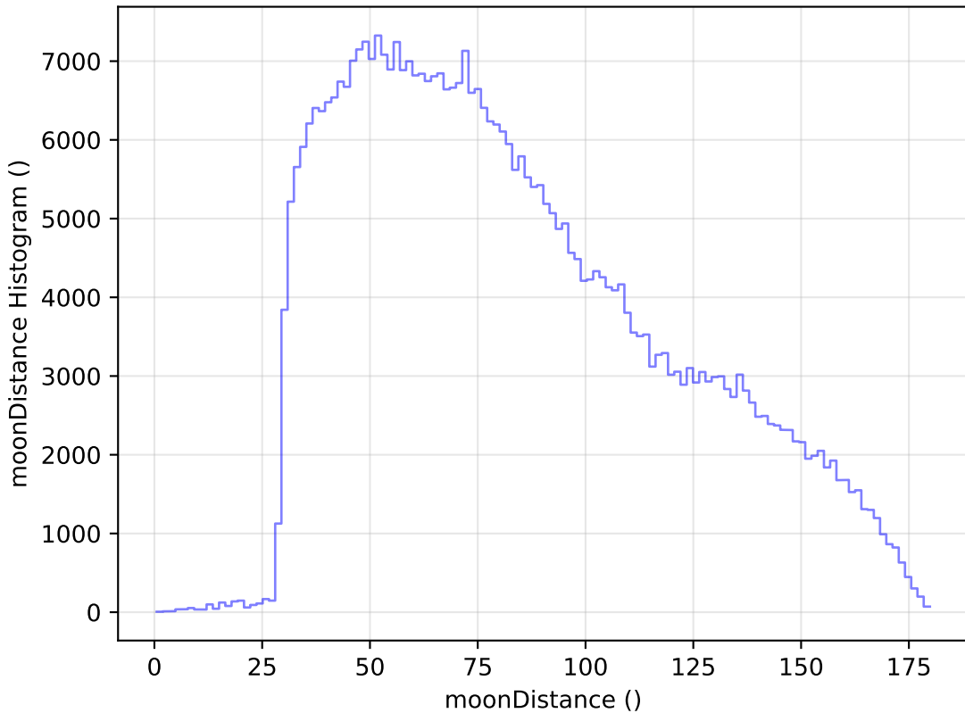
too_elab_r16_d2_griz_v3.4_10yrs WFD z band: moonDistance Histogram
