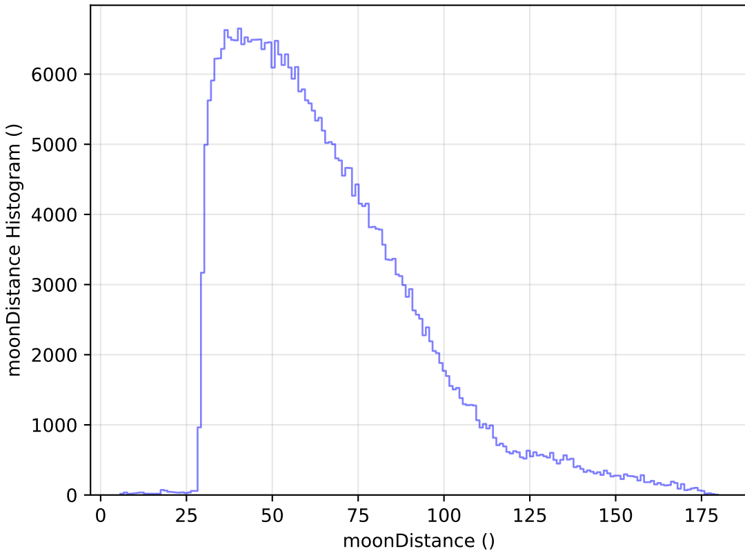
too_elab_r16_d2_griz_v3.4_10yrs WFD y band: moonDistance Histogram
