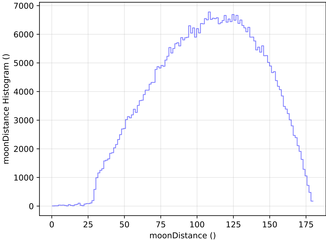
too_elab_r16_d2_griz_v3.4_10yrs WFD r band: moonDistance Histogram
