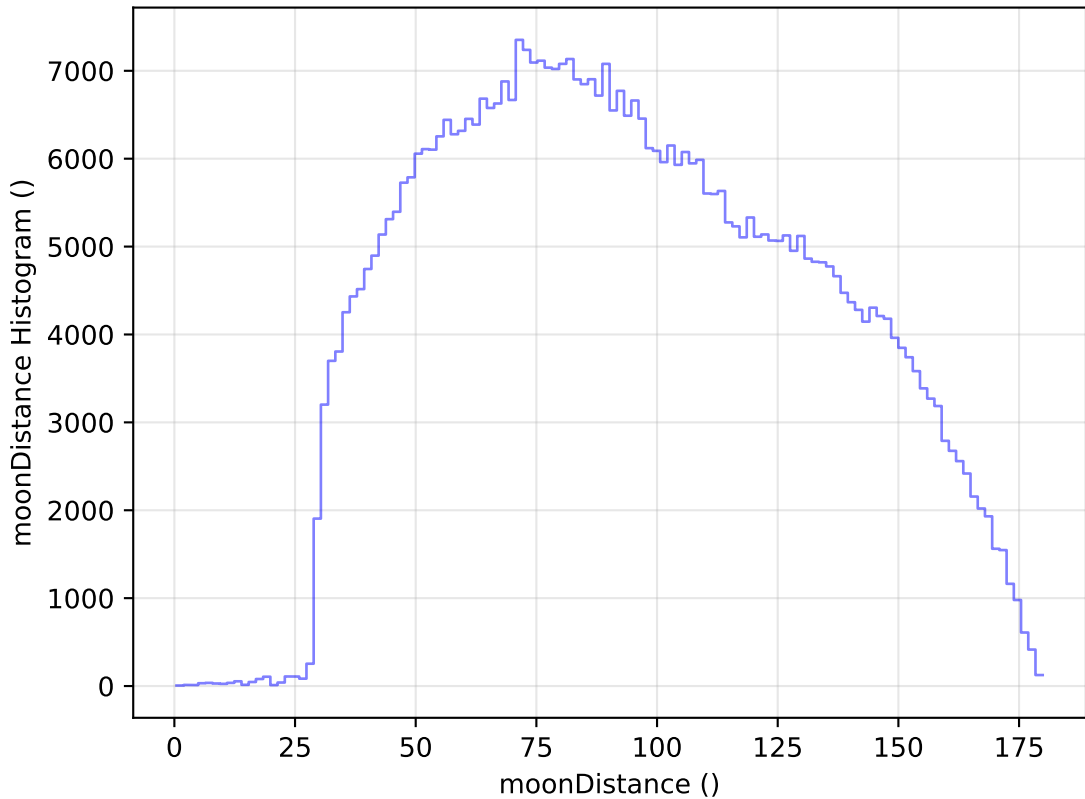
too_elab_r16_d2_griz_v3.4_10yrs WFD i band: moonDistance Histogram
