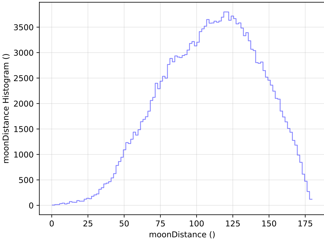
too_elab_r16_d2_griz_v3.4_10yrs WFD g band: moonDistance Histogram
