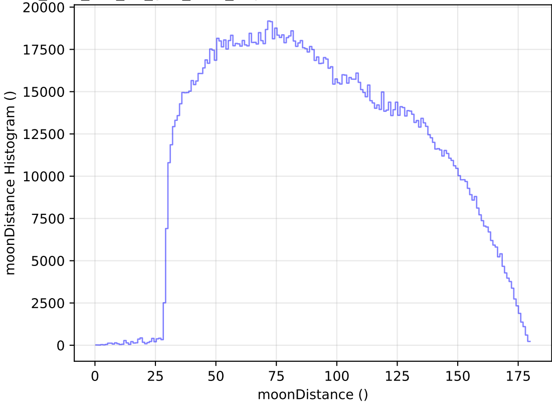
too_elab_r16_d2_griz_v3.4_10yrs WFD all bands: moonDistance Histogram
