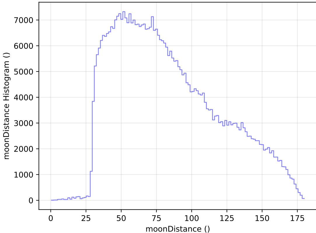
too_elab_r16_d2_griz_v3.4_10yrs All sky z band: moonDistance Histogram
