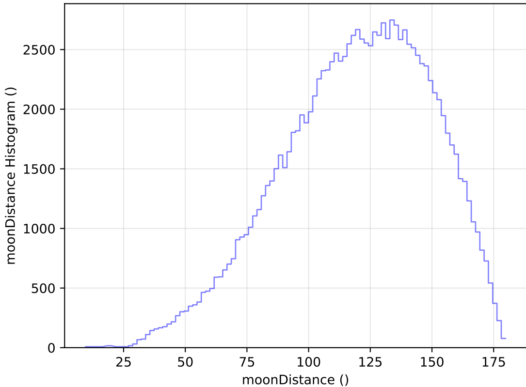
too_elab_r16_d2_griz_v3.4_10yrs All sky u band: moonDistance Histogram
