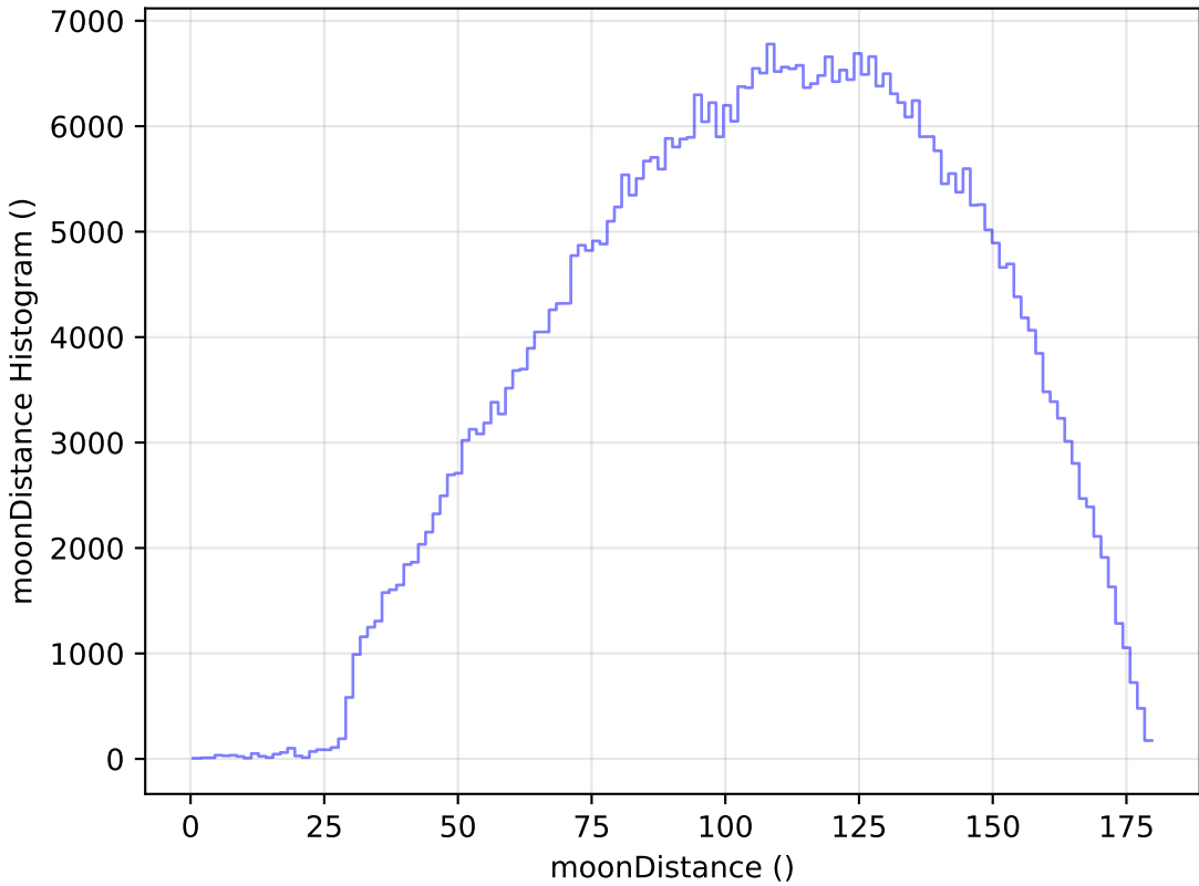
too_elab_r16_d2_griz_v3.4_10yrs All sky r band: moonDistance Histogram
