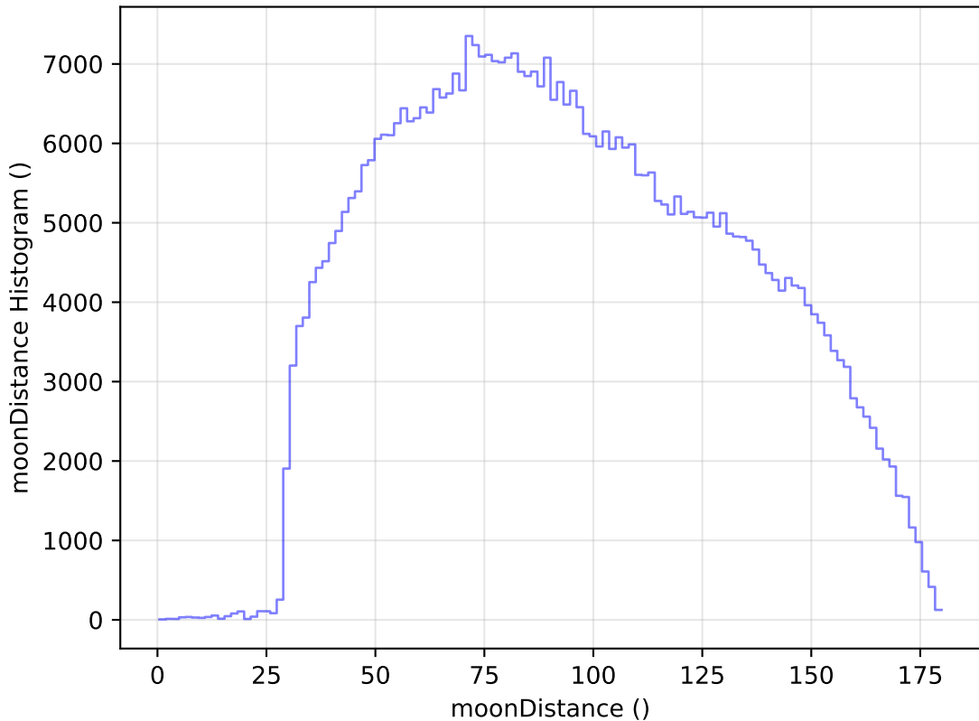
too_elab_r16_d2_griz_v3.4_10yrs All sky i band: moonDistance Histogram
