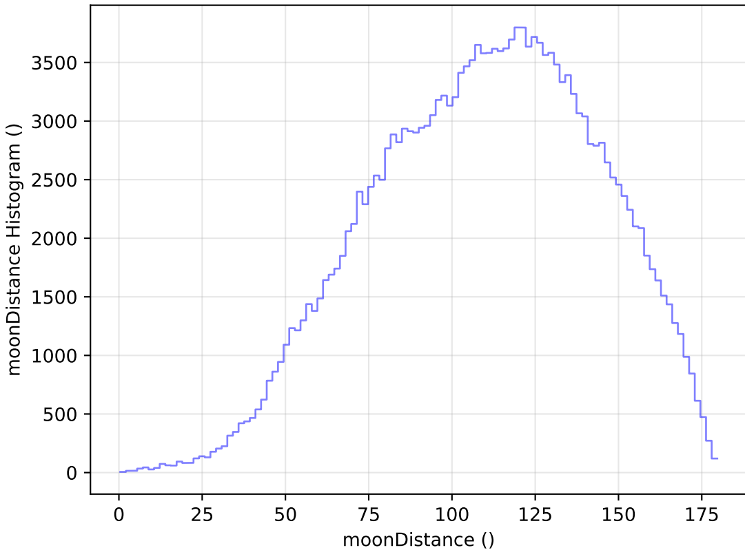
too_elab_r16_d2_griz_v3.4_10yrs All sky g band: moonDistance Histogram
