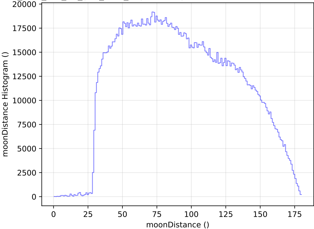
too_elab_r16_d2_griz_v3.4_10yrs All sky all bands: moonDistance Histogram
