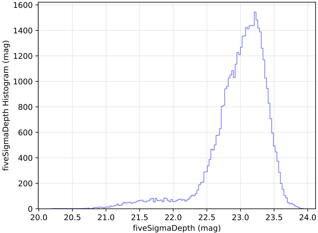
too_elab_r16_d2_griz_v3.4_10yrs Yr 1 z band: fiveSigmaDepth Histogram
