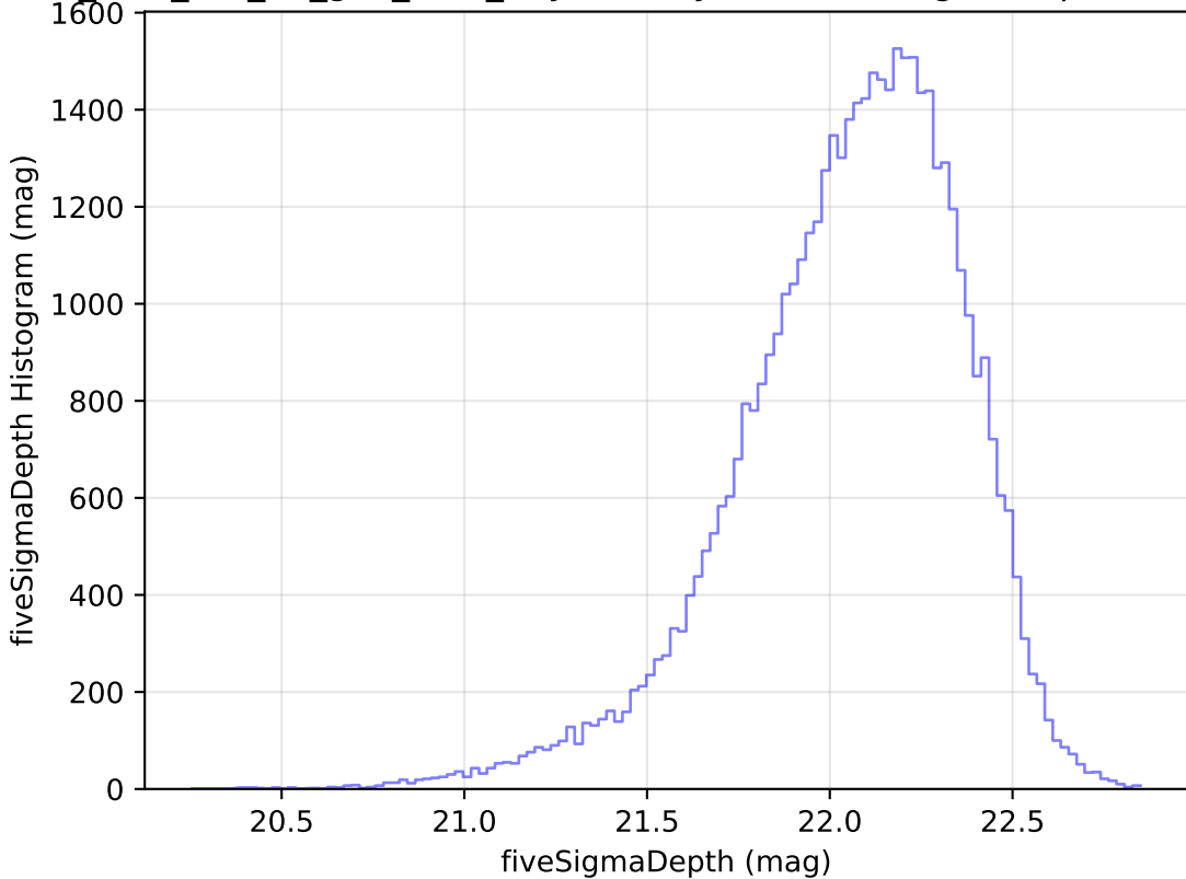
too_elab_r16_d2_griz_v3.4_10yrs Yr 1 y band: fiveSigmaDepth Histogram
