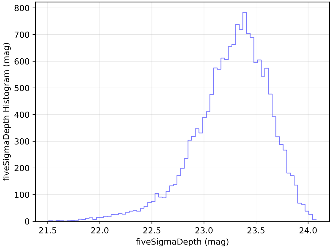
too_elab_r16_d2_griz_v3.4_10yrs Yr 1 u band: fiveSigmaDepth Histogram
