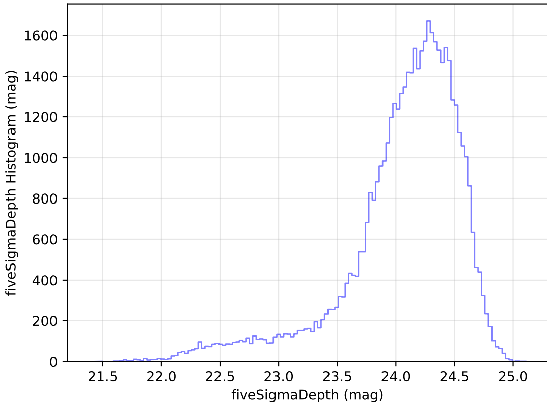
too_elab_r16_d2_griz_v3.4_10yrs Yr 1 r band: fiveSigmaDepth Histogram
