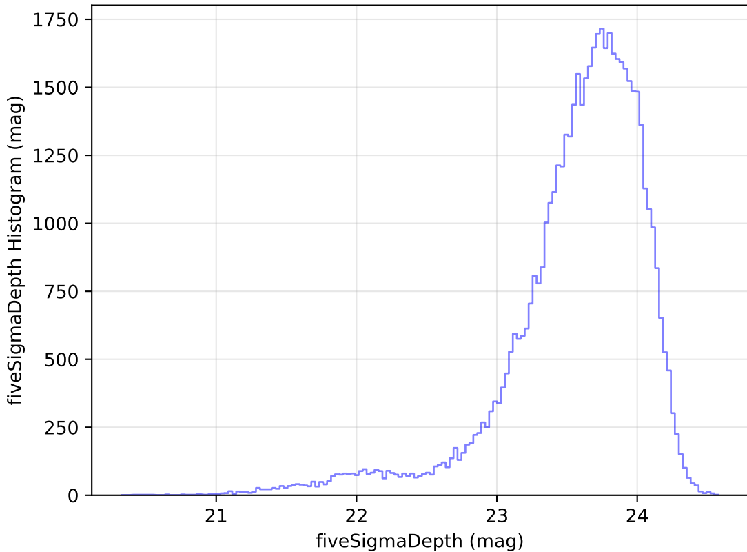
too_elab_r16_d2_griz_v3.4_10yrs Yr 1 i band: fiveSigmaDepth Histogram
