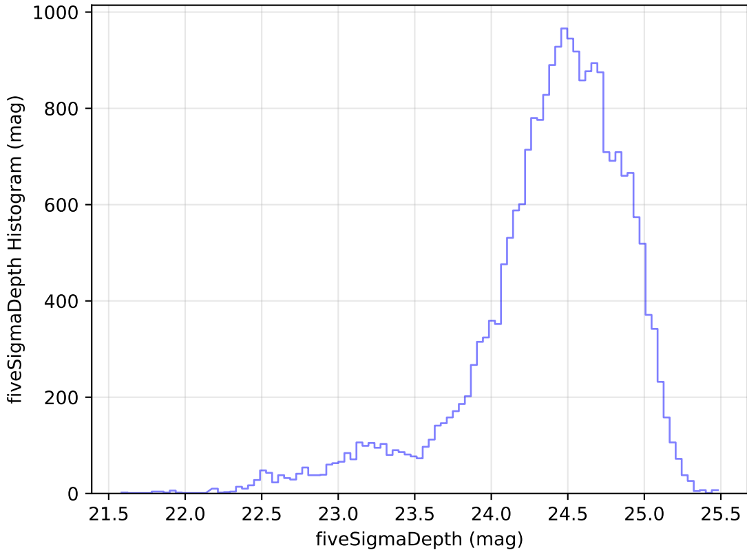
too_elab_r16_d2_griz_v3.4_10yrs Yr 1 g band: fiveSigmaDepth Histogram
