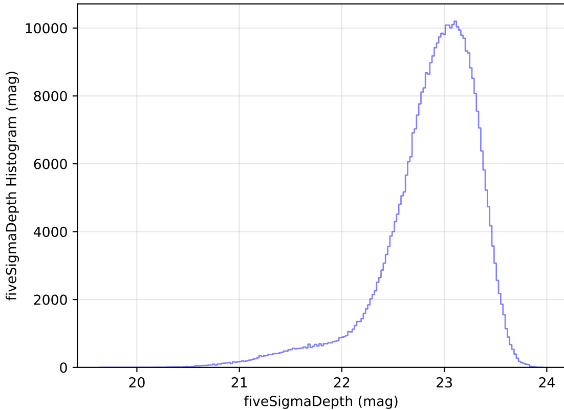
too_elab_r16_d2_griz_v3.4_10yrs WFD z band: fiveSigmaDepth Histogram
