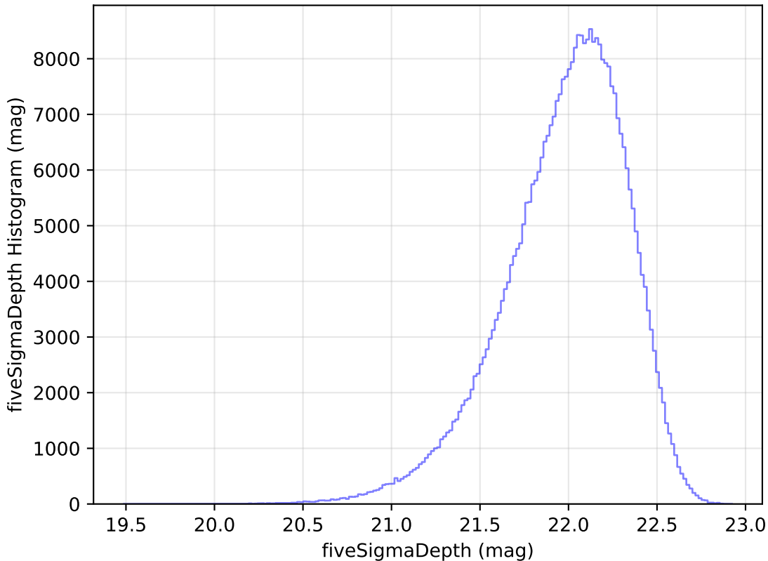
too_elab_r16_d2_griz_v3.4_10yrs WFD y band: fiveSigmaDepth Histogram
