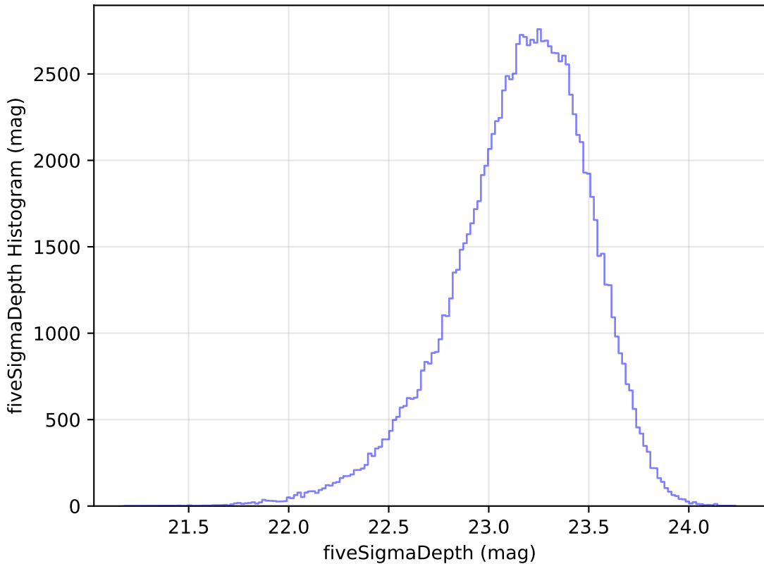
too_elab_r16_d2_griz_v3.4_10yrs WFD u band: fiveSigmaDepth Histogram
