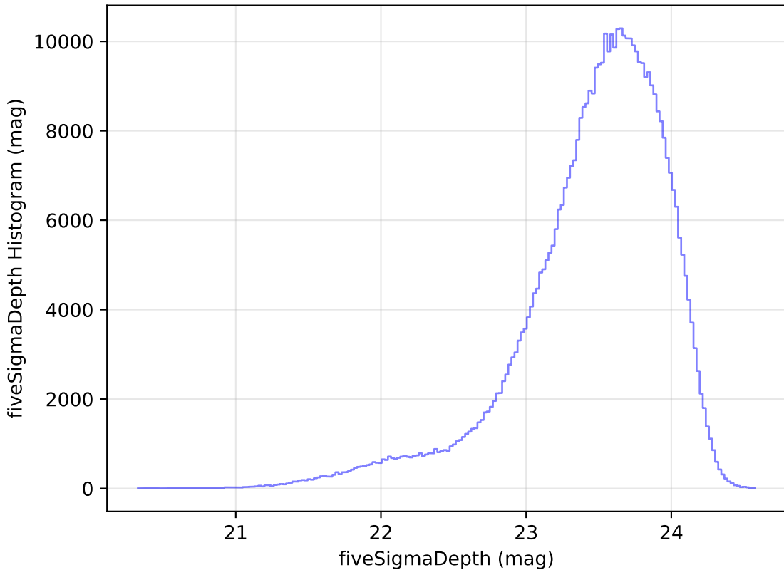
too_elab_r16_d2_griz_v3.4_10yrs WFD i band: fiveSigmaDepth Histogram
