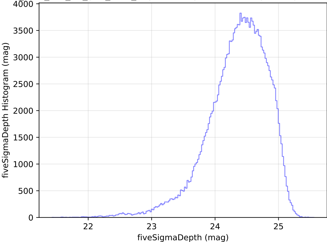
too_elab_r16_d2_griz_v3.4_10yrs WFD g band: fiveSigmaDepth Histogram
